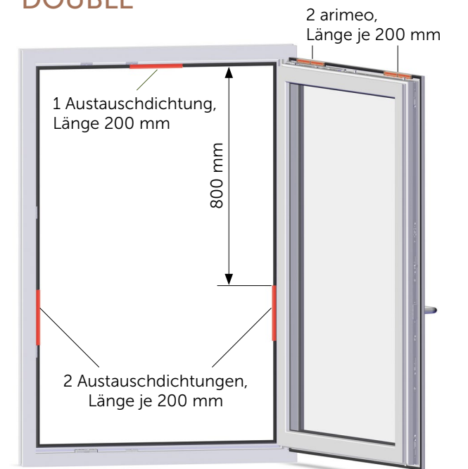
DOUBLE
