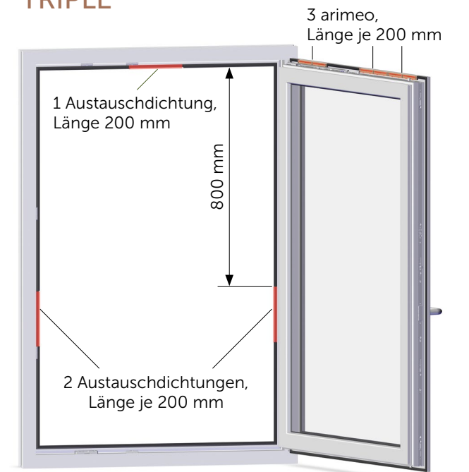
TRIPLE
