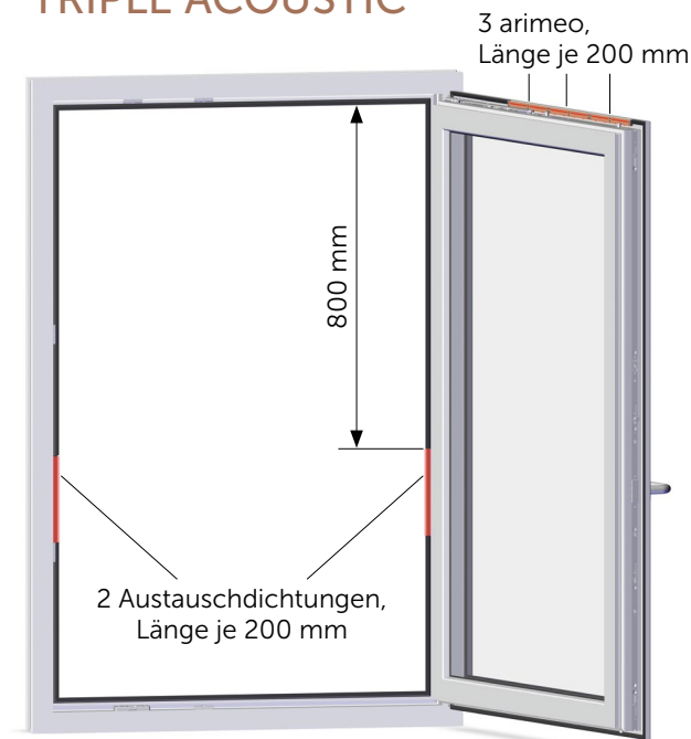
TRIPLE ACOUSTIC
