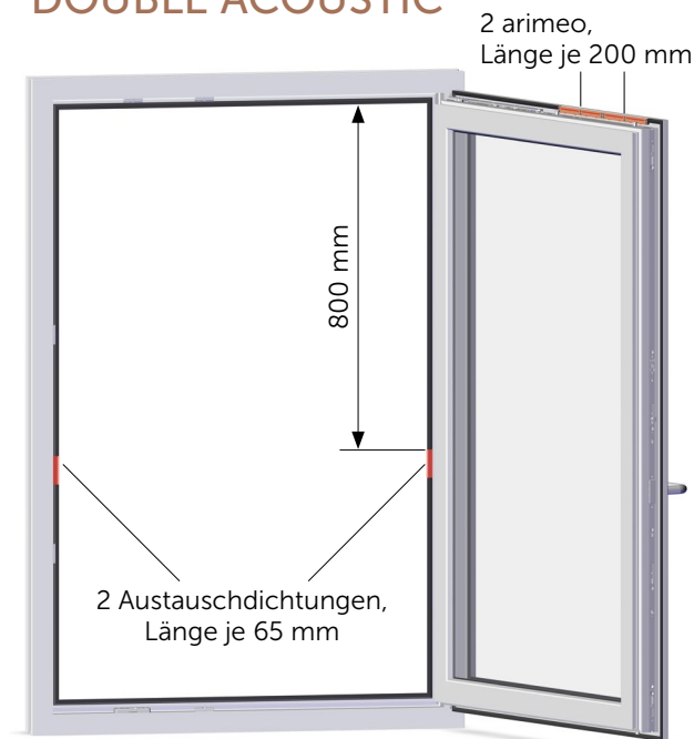
DOUBLE ACOUSTIC
