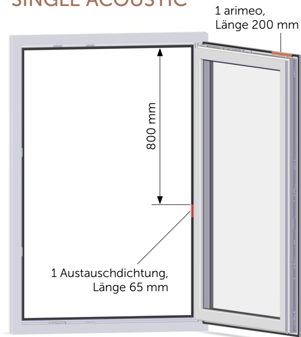
SINGLE ACOUSTIC
